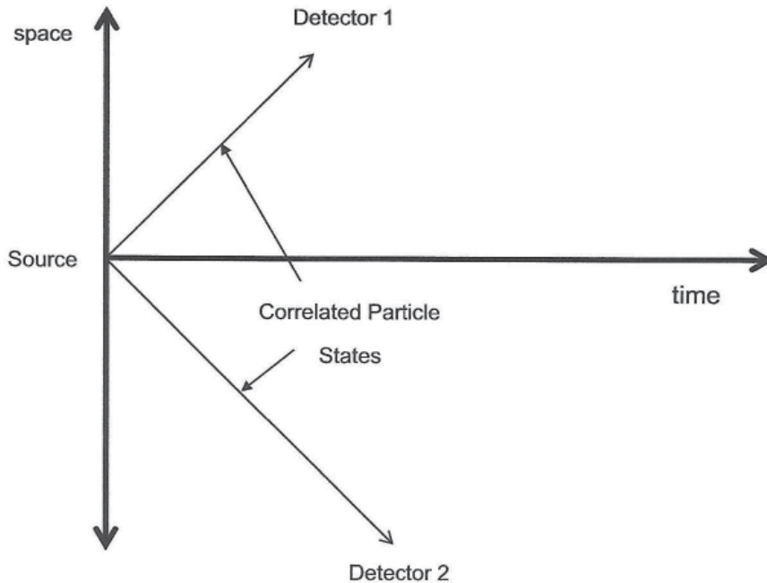
Figure 1. Space-time diagram of two entangled particles departing from a common source and moving apart in opposite directions in space and forward in time.
